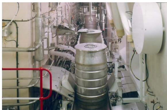
Encapsulation line at Sellafield Waste Packaging and Encapsulation Plant (WPEP)
